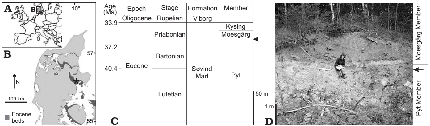
Fig. 1. A. Location of the studied area in Europe. B. Geological map (modified from Schwarzahns 2007: fig. 1) showing distribution of Eocene beds (dark gray) and location of the Eocene megachasmid locality (asterisk) in Moesgård Strand, Denmark. C. Generalized stratigraphy of the upper Paleogene marine deposits in Denmark (based on Thomsen et al. 2012). D. Photograph of the locality taken in 1988 by DJW with Alison Ward as a scale. The arrow in C, D points to bulk-sampled horizon that yielded the Eocene megachasmid tooth.
